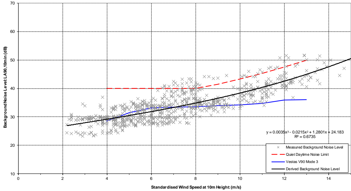
Chart 1 : Lower Foel Quiet Daytime Predicted Noise Levels and Noise Limit
